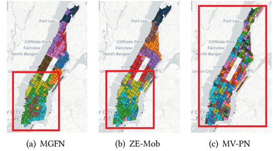
Figure 10: Visualization of clustering results in borough of Manhattan, NYC. Red squares mark where baselines perform worse than our model.
