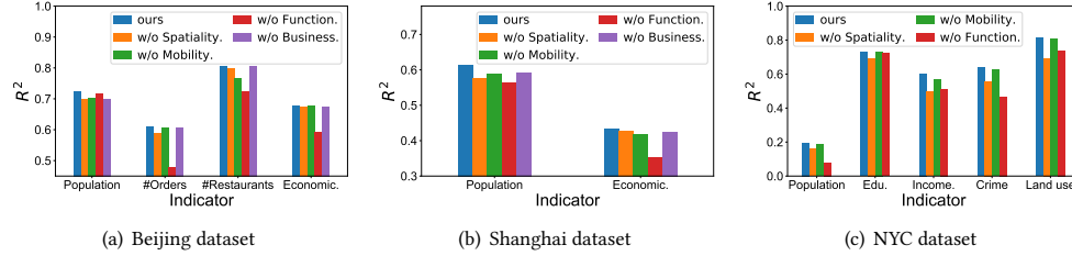
Figure 5: Performance comparison of models without specific domain knowledge.
