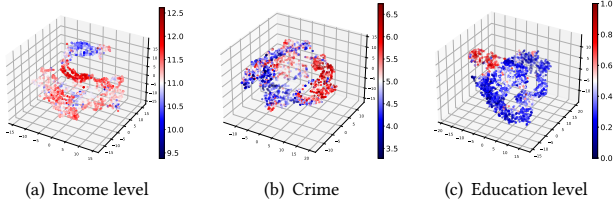
Figure 6: Visualization of location embeddings, where color represents the value of indicators. (Income level and crime are measured on log scale.)
