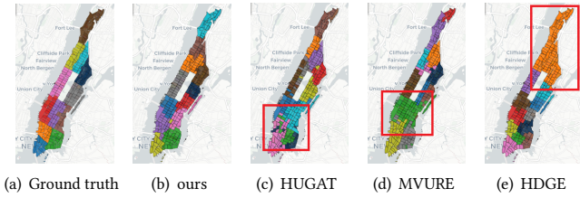
Figure 7: Visualization of clustering results in borough of Manhattan, NYC. Red squares mark where baselines perform worse than our model.
